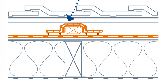
30 CM DIFFLEX THERMO ND (CLASSE 1)
